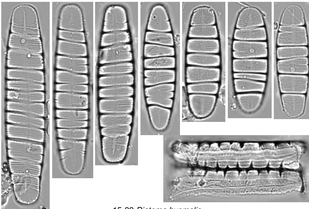
15-22 Diatoma hyemalis
