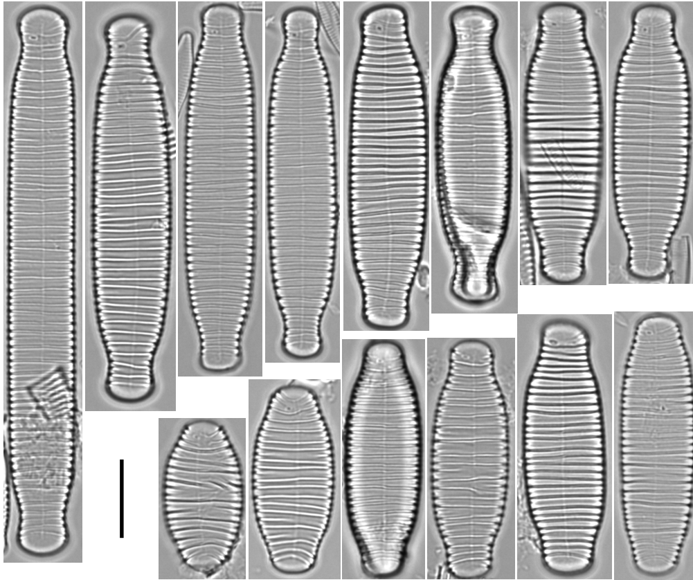
1-14 Diatoma ehrenbergii
