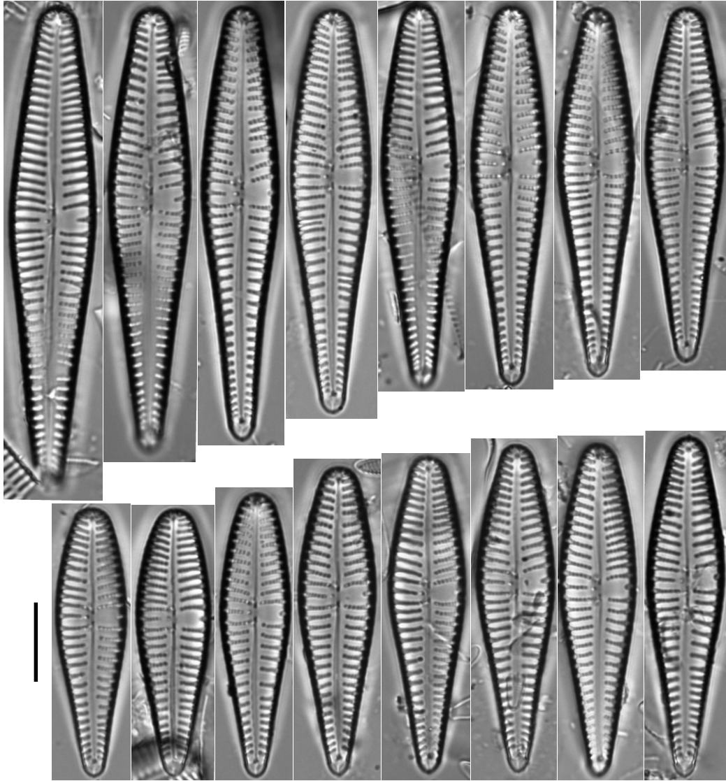
1-16 Gomphonema zellense
