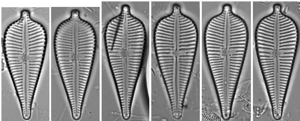
17-22 Gomphonema augur
