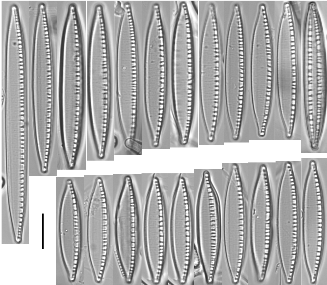
1-22 Nitzschia sp. 2
