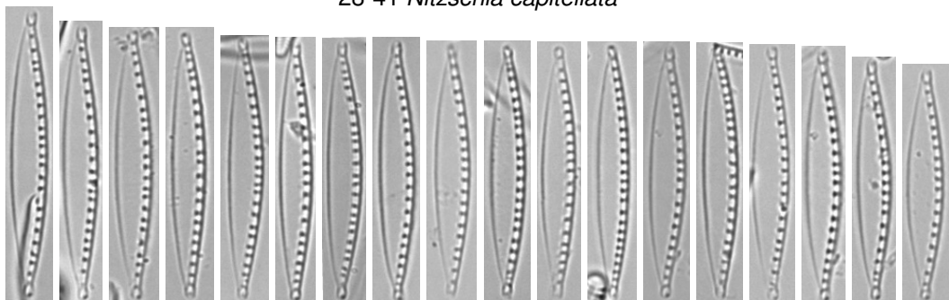
42-59 Nitzschia sociabilis
